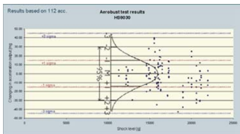
Fig 6 : Bias shift due to Aerobutt firing test, ranging from 11'000 g to 22'000 g's along 3 axis
