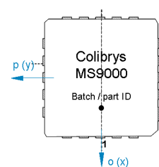
MS9000 top view
