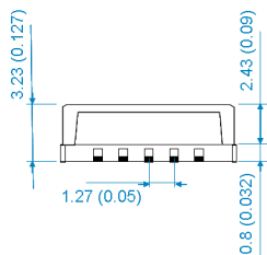
VS9000 side view
