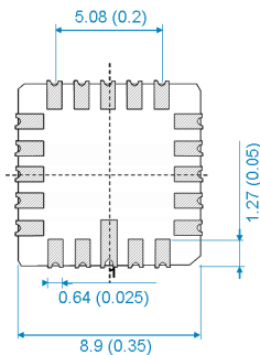
VS9000 bottom view
