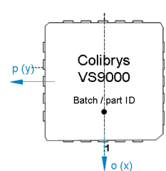
VS9000 top view
